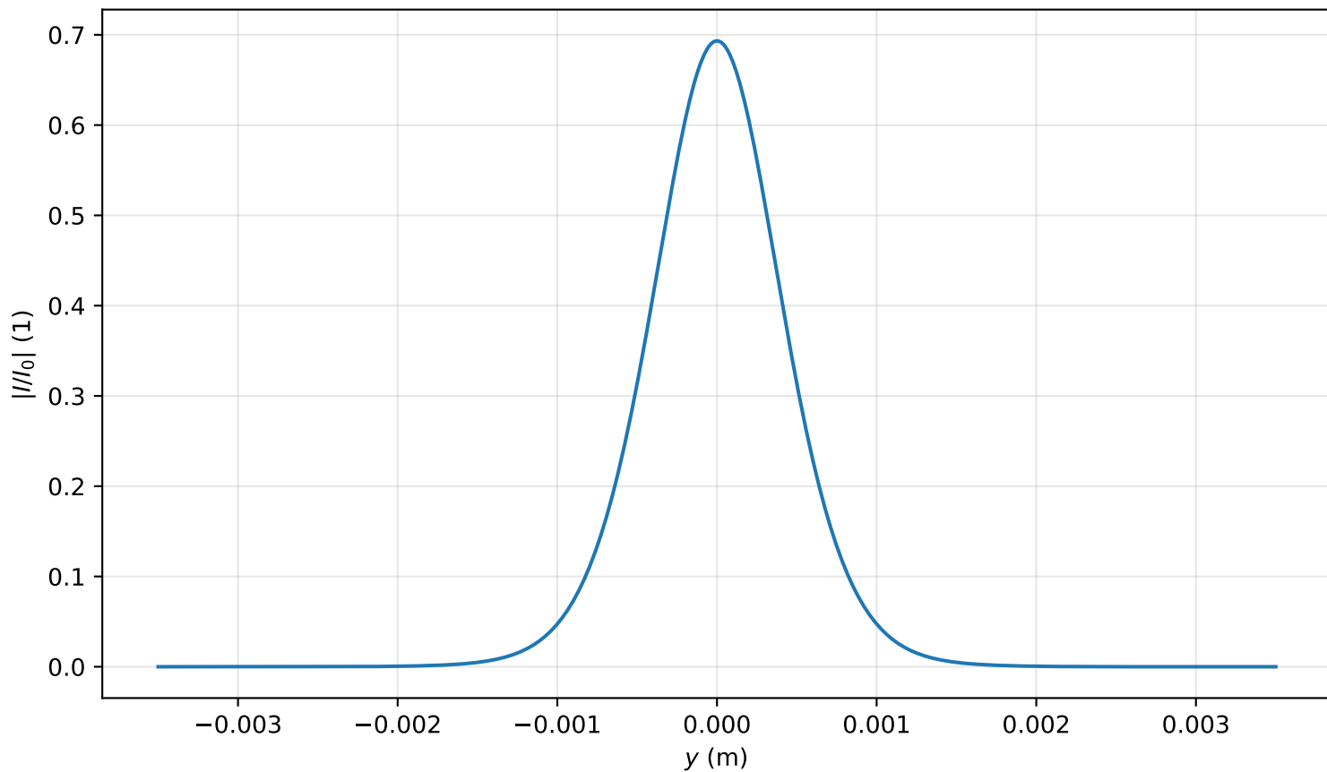
Intensity profile I(x=0, y, z=2.468)/I_0 , \text{Pin}=0.5P_{\text{cr}} , artificial time
